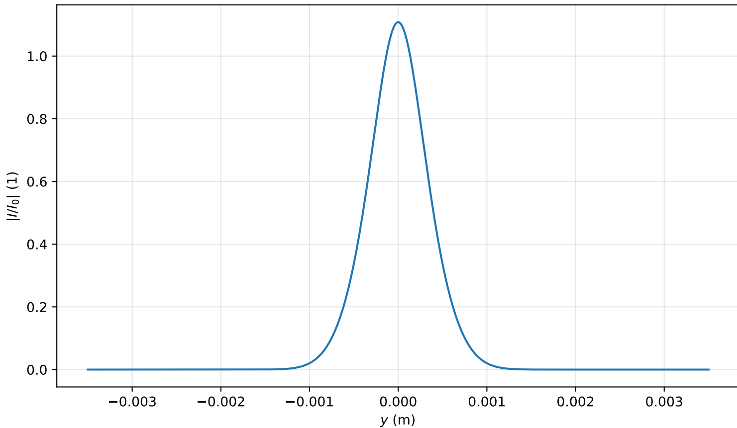
Intensity profile I(x=0, y, z=0.557)/I_0 , \text{Pin}=0.7\text{Pcr} , artificial time
